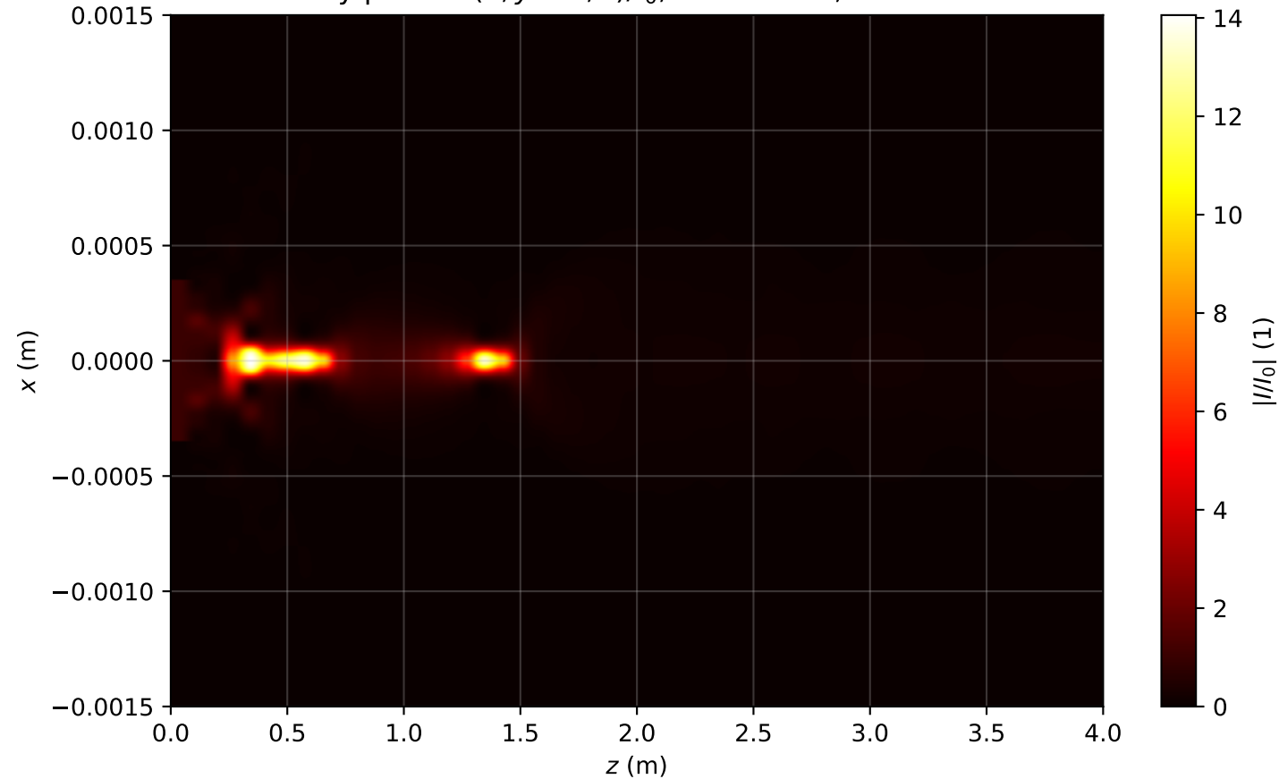
Intensity profile I(x, y = 0, z)/I_0 , P_{in}=5.0P_{cr} , artificial time
